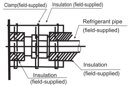
Piping insulation procedure
